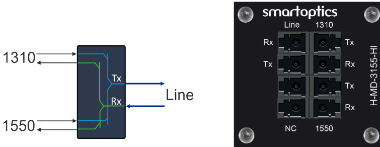
Figure 66: H-MD-3155 icon and front plate
