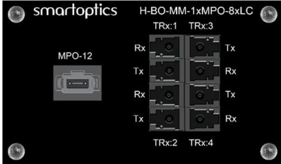
Figure 76: Front of H-BO-MM-1xMPO-8xLC
