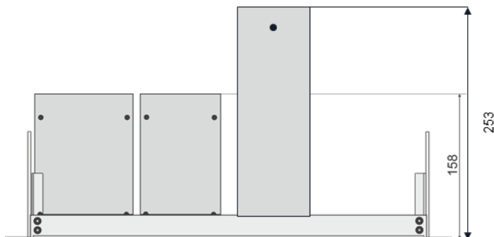
Figure 87: Top view of two H-Series filter and one H-PPM-CHASSI-1 module mounted in H-CHASSI-1RU. The length of the H-PPM-CHASSI-1 is longer, making it extend the standard module depth.
