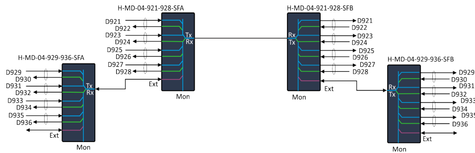
Figure 56: 8ch configuration
