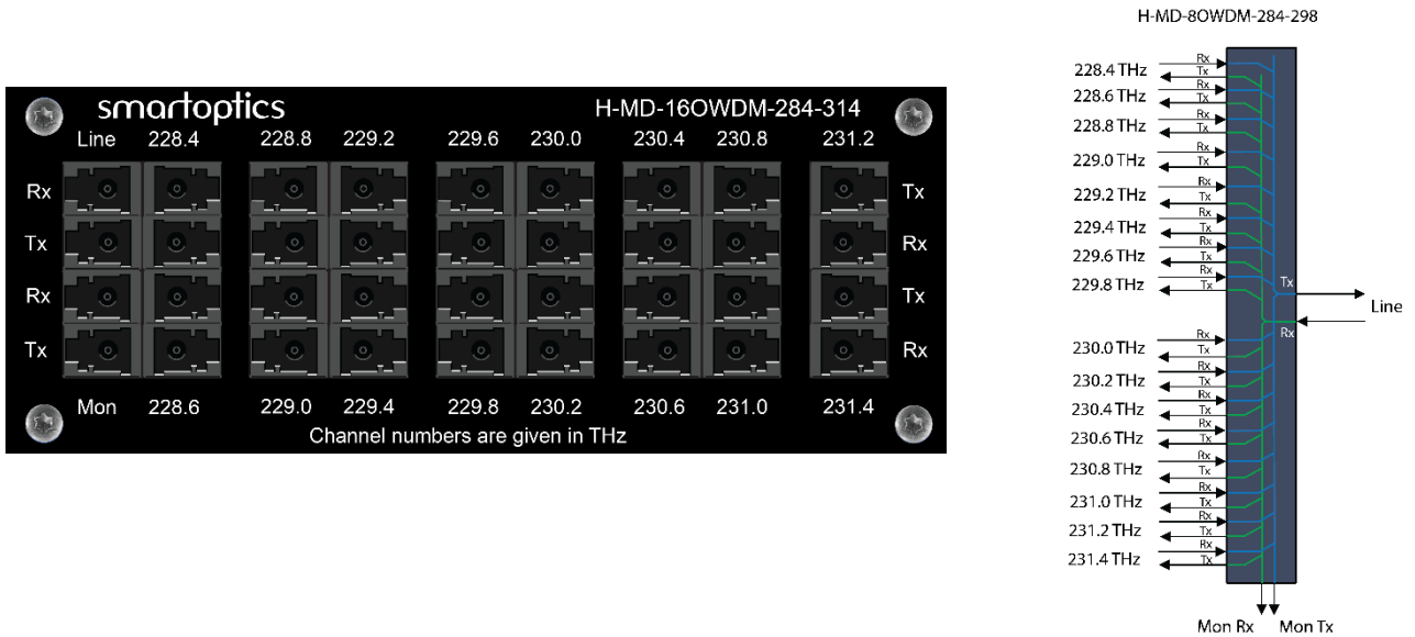
Figure 61: H-MD-16OWDM-384-314 icon and front plate
