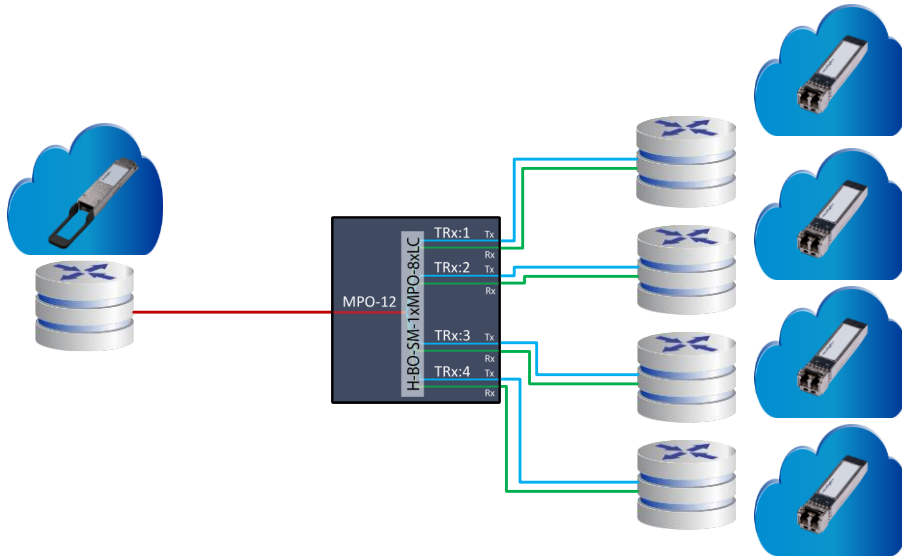
Figure 78: Illustrative application of H-BO-MM-1xMPO-8xLC
