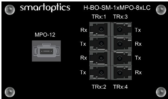
Figure 73: Front of H-BO-SM-1xMPO-8xLC
