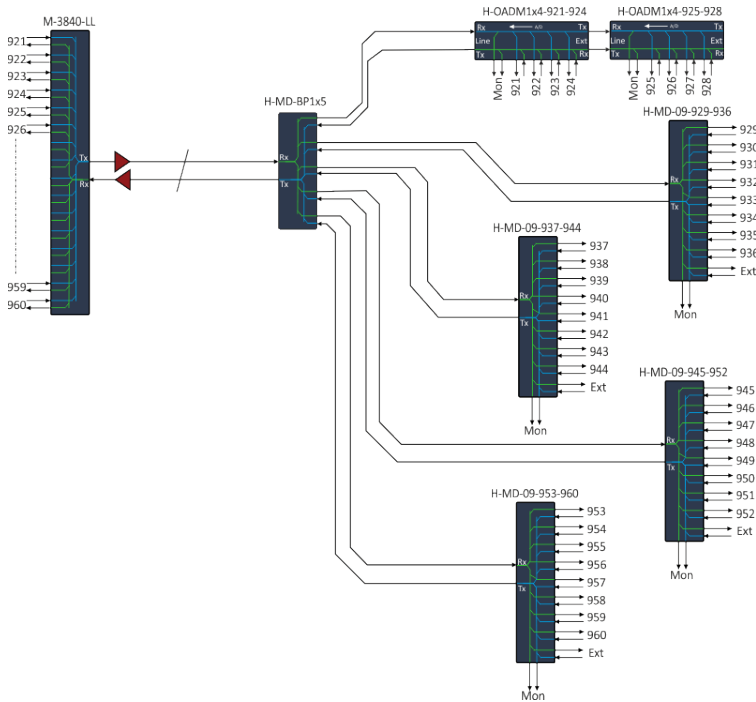
Figure 49: Example configuration
