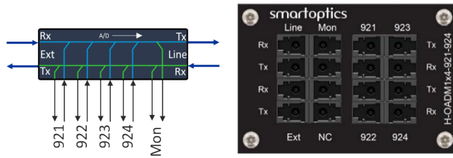
Figure 38: H-OADM1x4-921-924 icon and front plate
