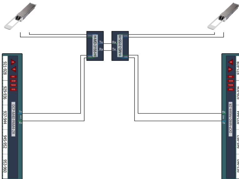
Figure 67: Mixed 1x 100G and Amplified DWDM configuration example
