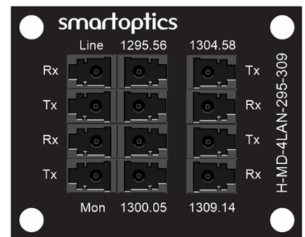
Figure 58: Front view of H-4LAN-295-309
