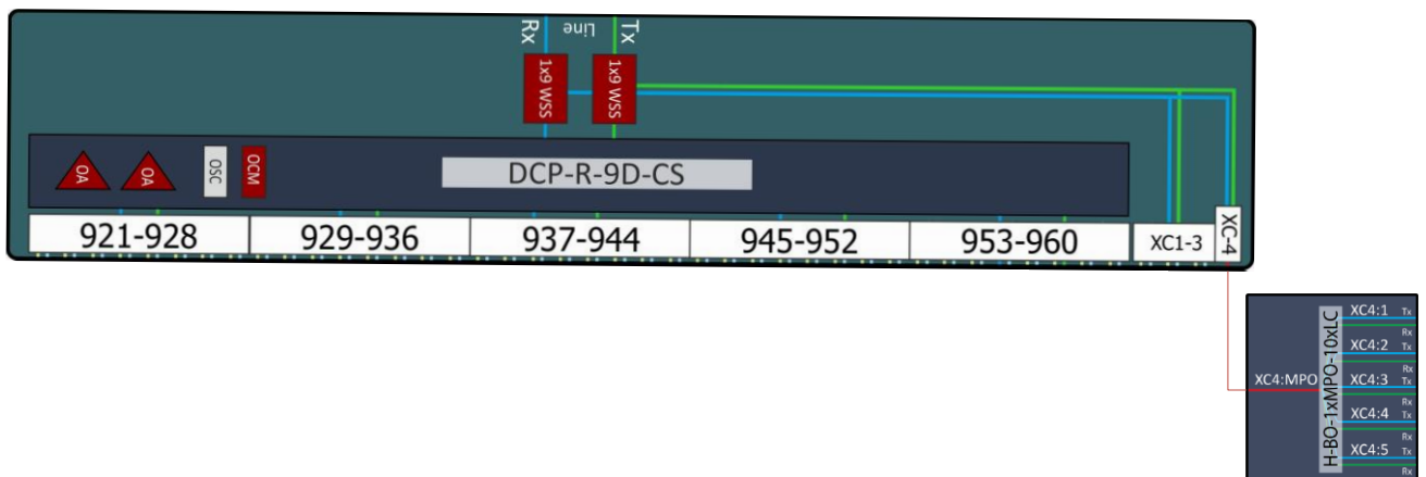
Figure 72: Illustration of breaking out the XC-4 MPO connector on the DCP-R9D-CS into five duplex LC ports
