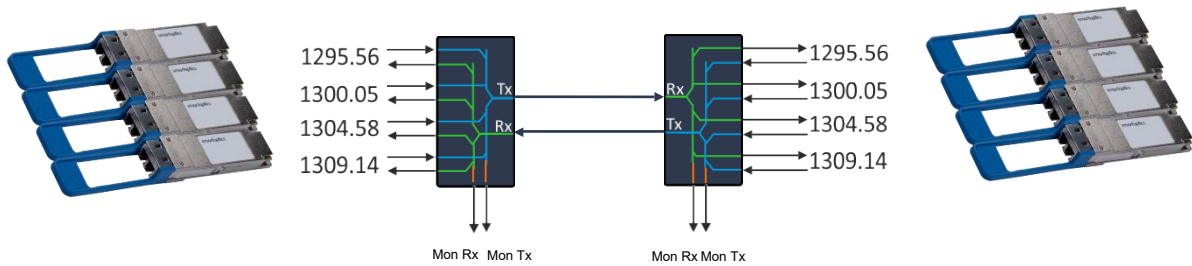
Figure 59: 4x100G configuration using 100G O-band DWDM transceivers
