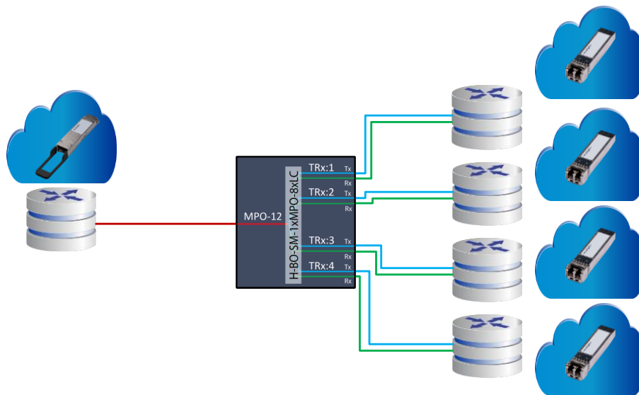
Figure 75: Illustrative application of H-BO-SM-1xMPO-8xLC
