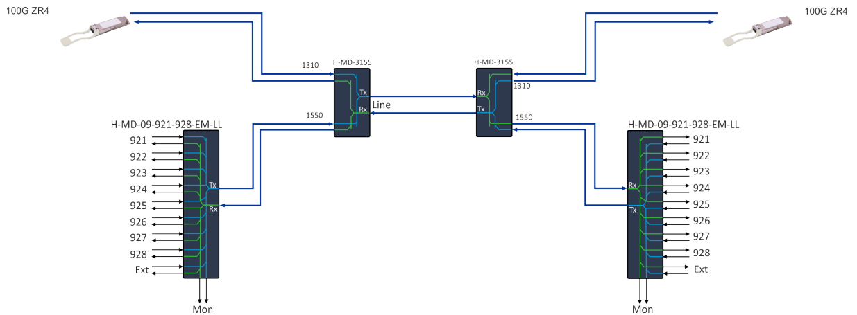
Figure 65: Mixed 1x 100G and DWDM configuration example
