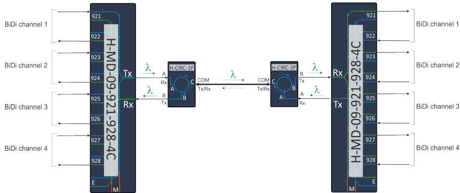
Figure 53: Single-fiber configuration example
