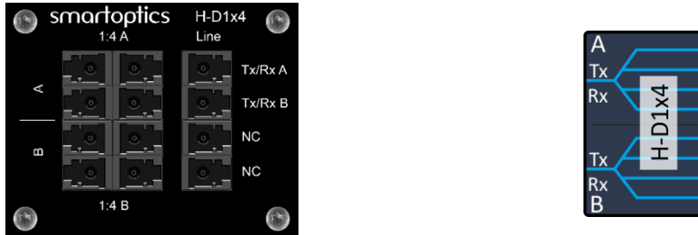
Figure 79: Front and logical icon of H-D1x4
