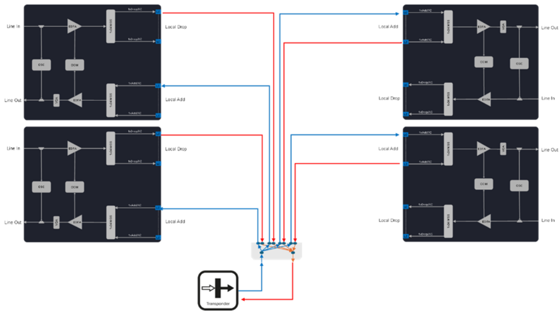
Figure 80: Functional Diagram of the H-D1x4 with a DCP-R
