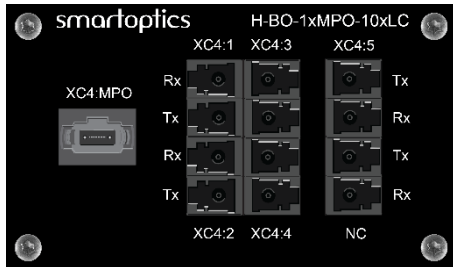
Figure 70: Front of H-BO-1xMPO-10xLC
