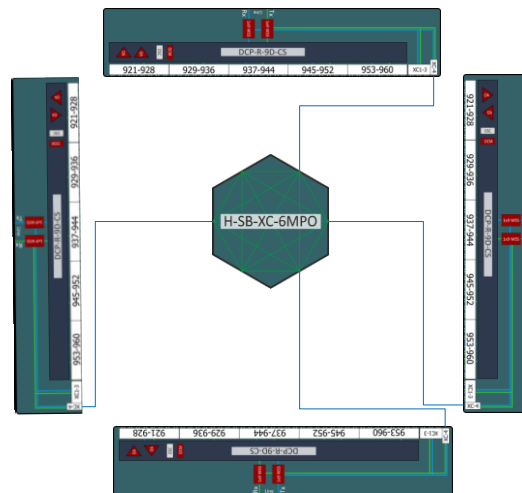
Figure 69: Illustration of how four DCP-R-9D-CS are interconnected through the H-SB-XC-6MPO
