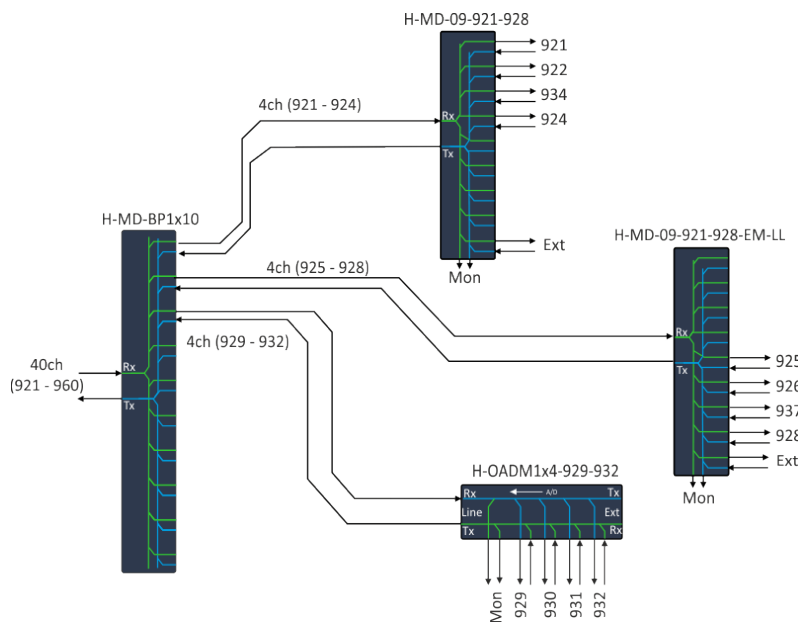
Figure 51: 10-way fan-out configuration.
