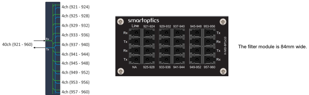
Figure 50: H-MD-BP1x10 icon and front plate
