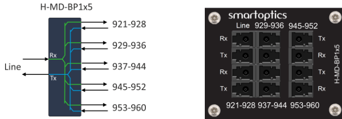
Figure 48: H-MD-BP1x5 icon and front plate
