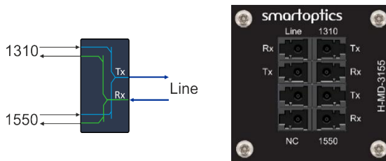
Figure 62: H-MD-3155 icon and front plate
