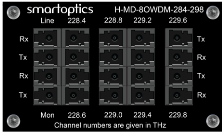
Figure 60: H-MD-8OWDM-284-298 icon and front plate
