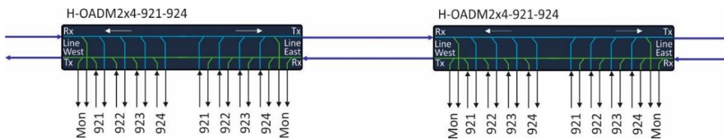
Figure 41: Two H-OADM2x4-921-924 filters connected in a bus configuration.
