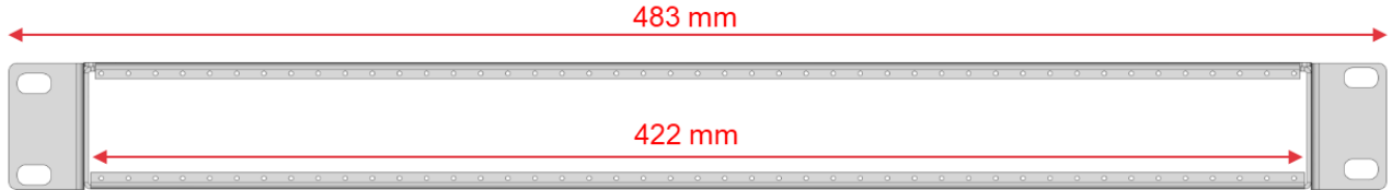
Figure 82: H-CHASSI-1RU
