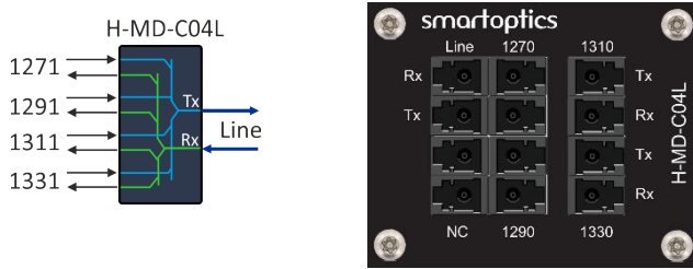
Figure 3: H-MD-C04L logical icon and front plate
