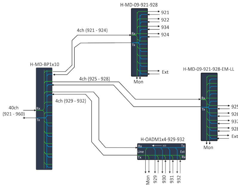
Figure 46: 10-way fan-out configuration.
