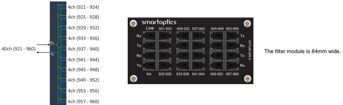
Figure 45: H-MD-BP1x10 icon and front plate
