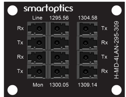
Figure 53: Front view of H-4LAN-295-309
