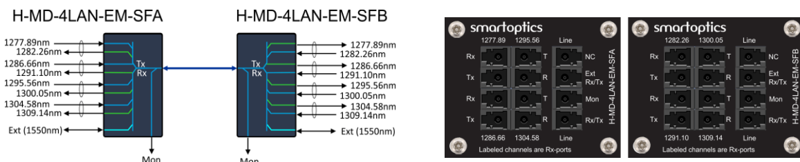
Figure 52: H-MD-4LAN-EM-SFx icons and front plates
