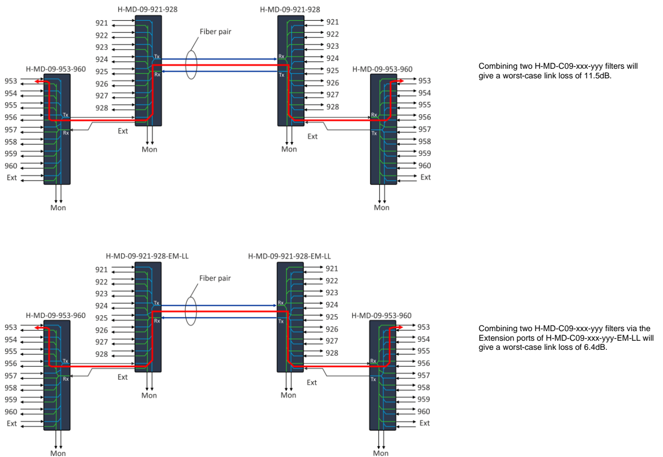
Figure 27: Configuration examples to show how the loss table above is used
