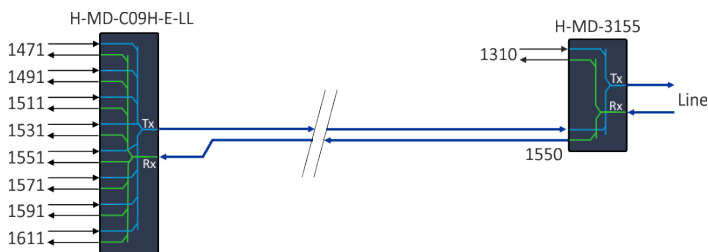
Figure 58: Mixed 1310nm legacy and CWDM configuration example
