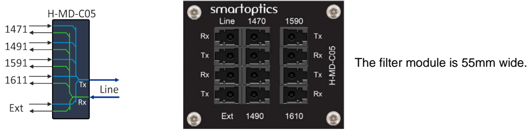
Figure 7: H-MD-C05 logical icon and front plate
