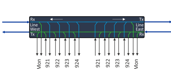
Figure 40: H-OADM2x4-921-924-4C icon and front plate
