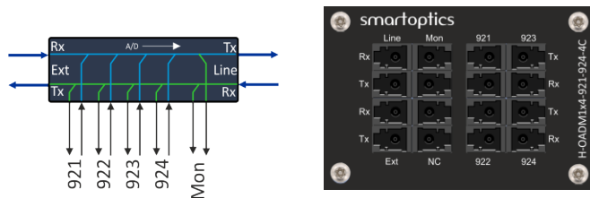
Figure 38: H-OADM1x4-921-924-4C icon and front plate
