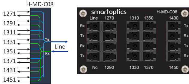
Figure 11: H-MD-C08 logical icon and front plate
