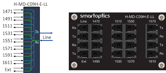
Figure 18: H-MD-C09H-E-LL logical icon and front plate
