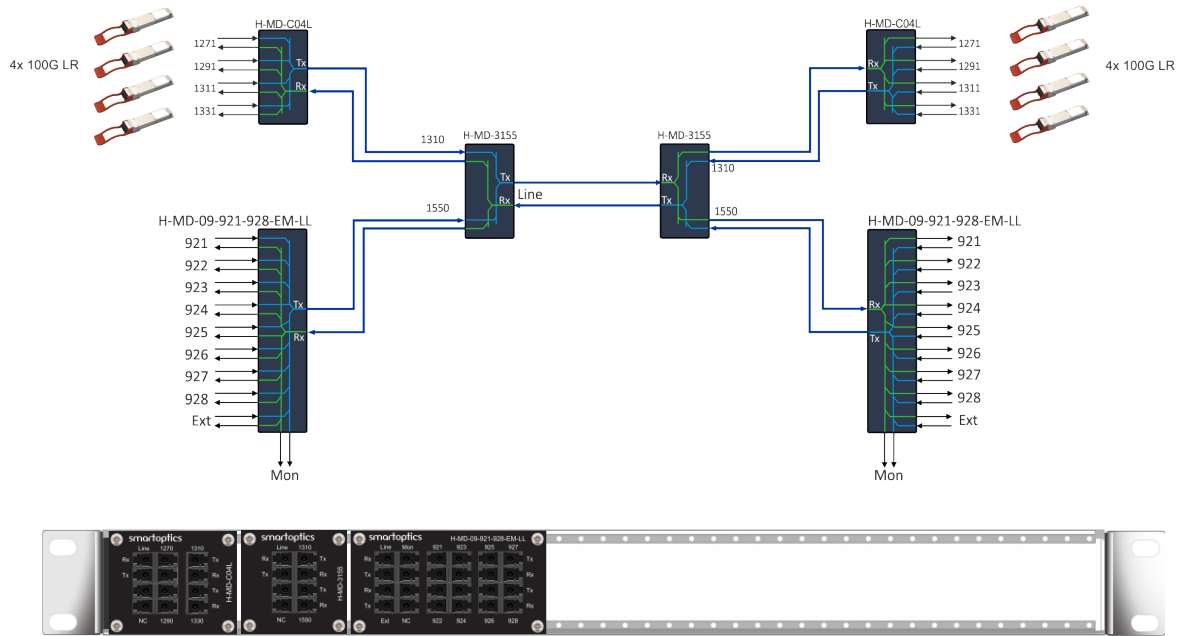
Figure 59: Mixed 4x 100G and DWDM configuration example
