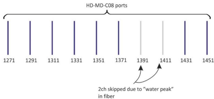
Figure 12: H-MD-C08 channels
