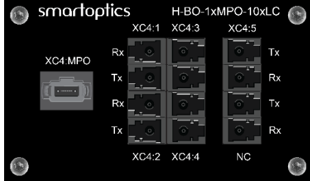
Figure 66: Front of H-BO-1xMPO-10xLC
