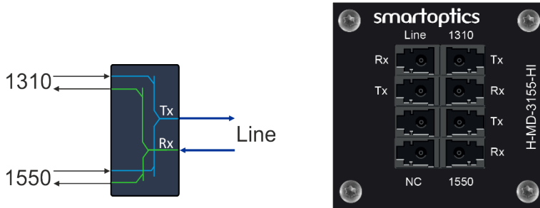
Figure 61: H-MD-3155 icon and front plate
