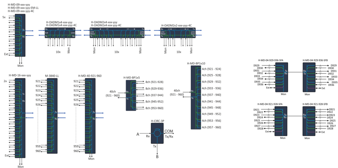
Figure 23: DWDM filters
