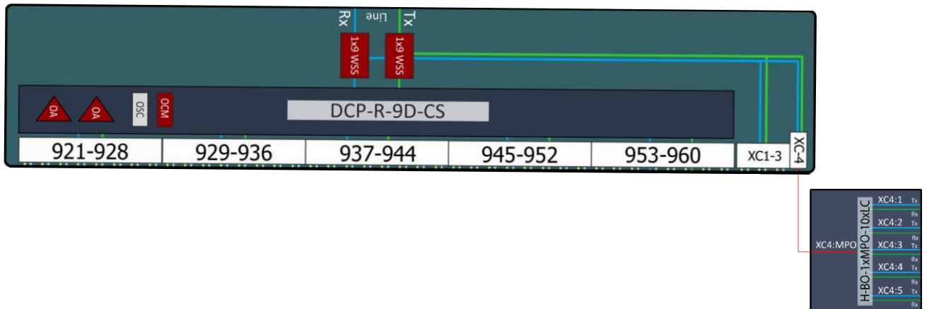
Figure 67: Illustration of breaking out the XC-4 MPO connector on the DCP-R9D-CS into five duplex LC ports
