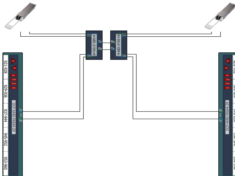
Figure 62: Mixed 1x 100G and Amplified DWDM configuration example
