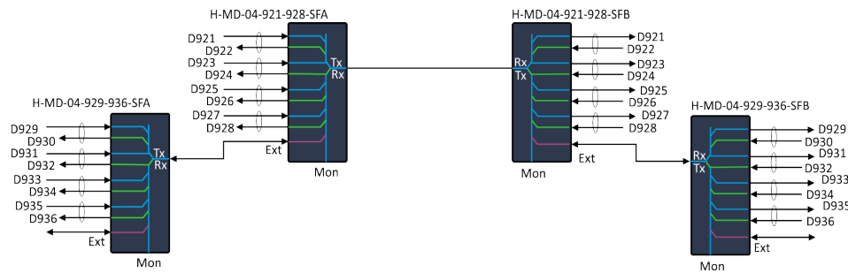
Figure 51: 8ch configuration
