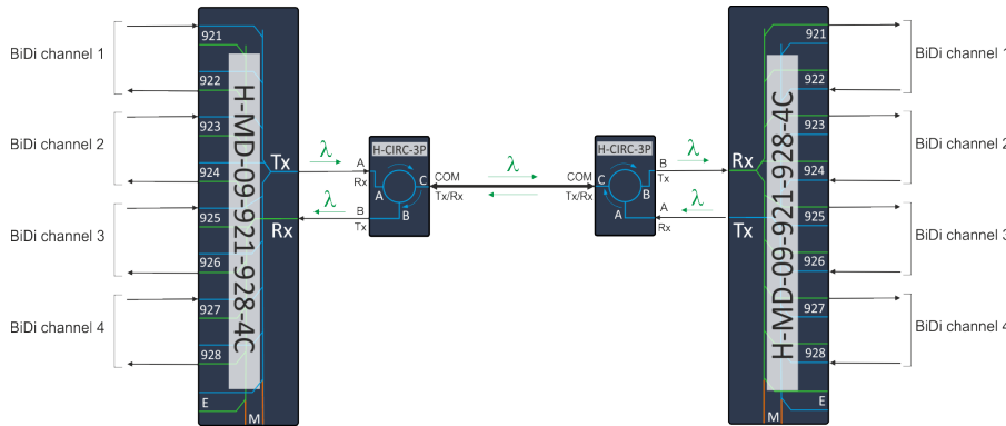
Figure 48: Single-fiber configuration example
