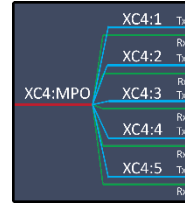
Figure 65: Logical Icon of H-BO-1xMPO-1xLC
