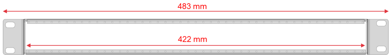
Figure 68: H-CHASSI-1RU
