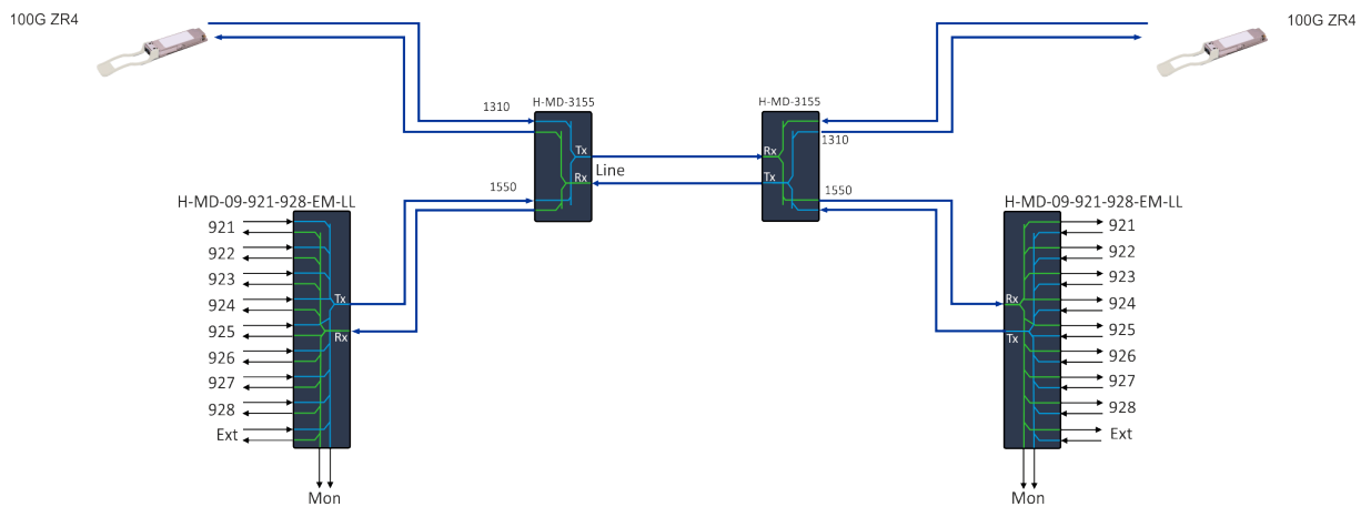
Figure 60: Mixed 1x 100G and DWDM configuration example
