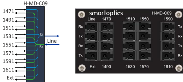
Figure 15: H-MD-C09 logical icon and front plate
