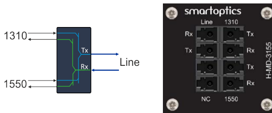
Figure 57: H-MD-3155 icon and front plate
