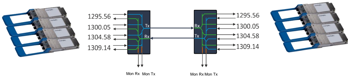
Figure 54: 4x100G configuration using 100G O-band DWDM transceivers
