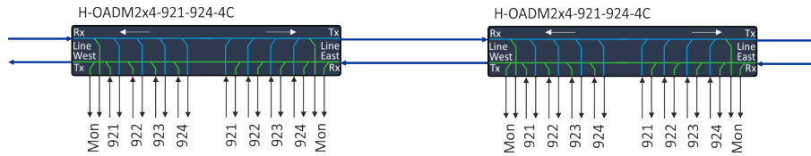
Figure 41: Two H-OADM2x4-921-924-4C filters connected in a bus configuration.
